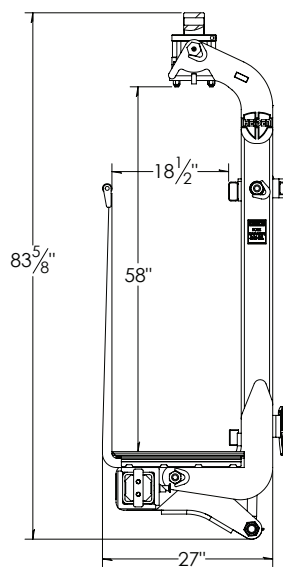
STOWED POSITION
