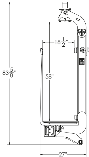
STOWED POSITION
